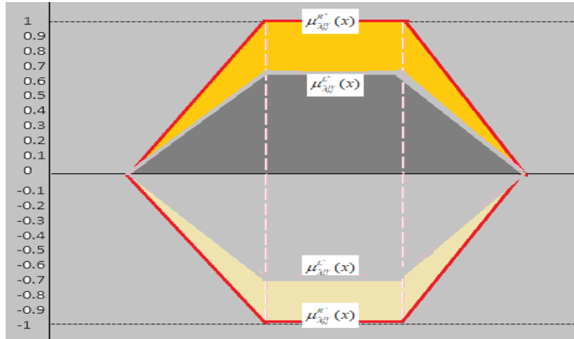
Figure 2. IVBSVTrFN.
