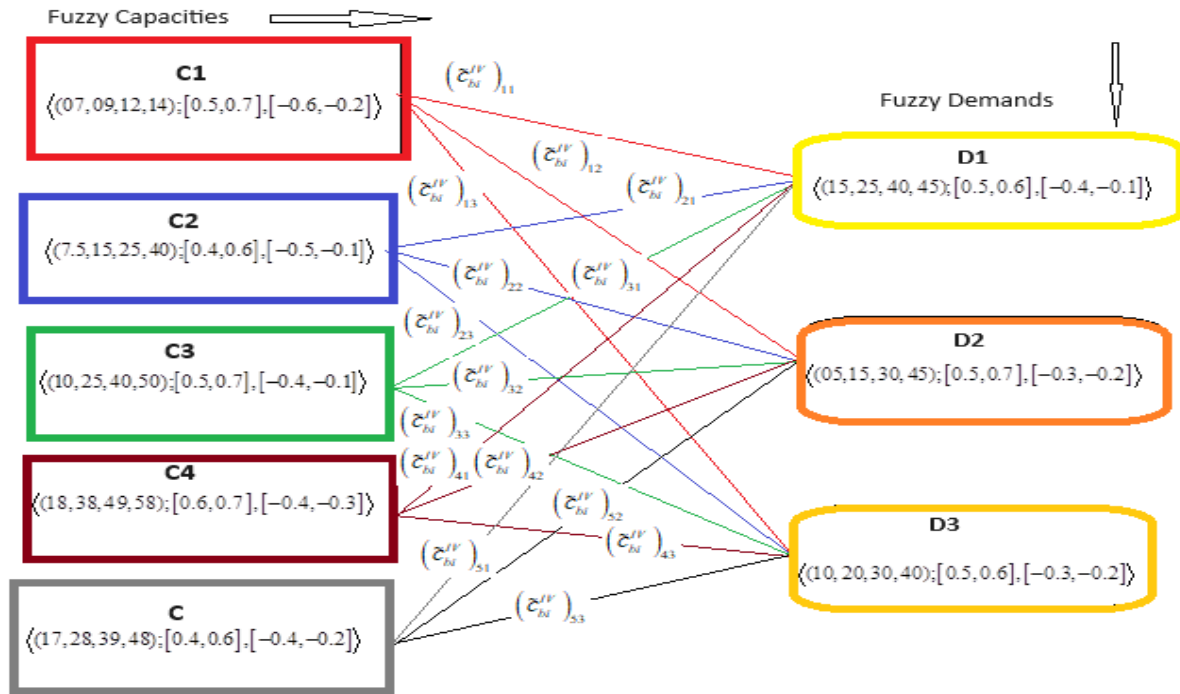
Figure 3. FFDPP.
