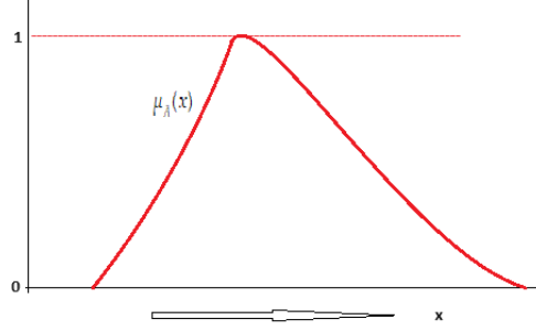
Figure 1. Fuzzy number.
