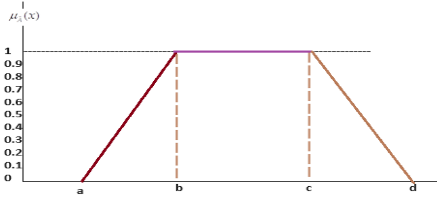
Figure 1. Trapezoidal fuzzy number.
